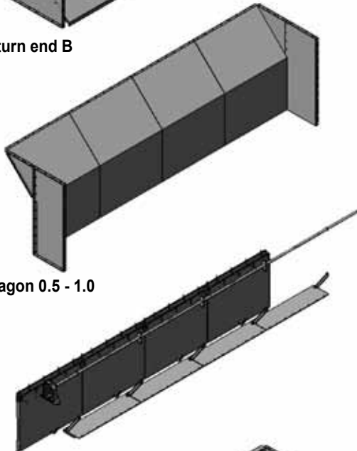
A70966 - bottom shutter B
