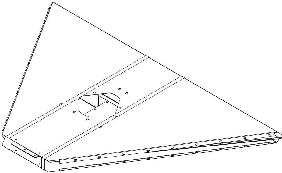
Base cone package A70374P - external dimensions 180 x 1240 x 1985 mm - weight 132 kg
